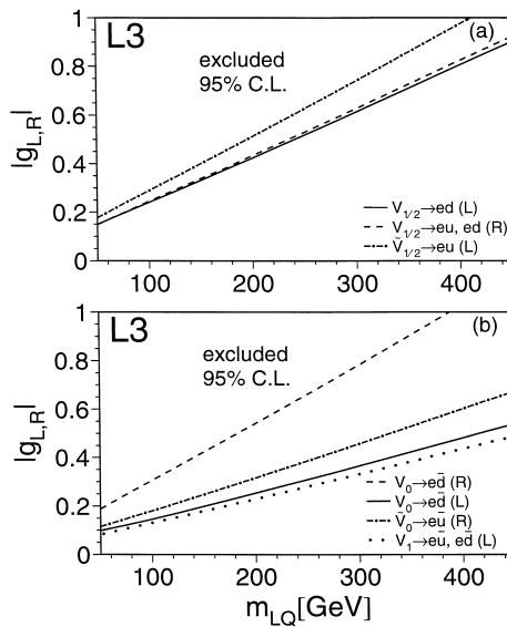
Fig. 5. The 95% confidence level upper limits on |g_{L,R}| as a function of m_{LQ} for various vector leptoquarks derived from hadronic cross sections. Limits are shown for fermion number F = 2 (a) and for F = 0 (b).
