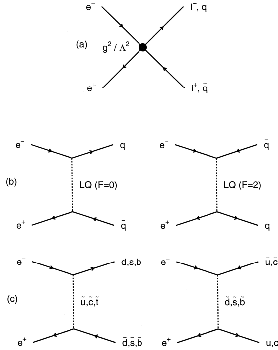
Fig. 1. a) Feynman diagram describing the contact interactions; (b) Feynman diagrams describing the t -channel exchange, left, and u -channel exchange, right, of leptoquarks with fermion number F = L + 3B ; (c) Feynman diagrams describing the t -channel exchange, left, and u -channel exchange, right, of scalar quarks.
