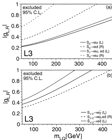
Fig. 4. The 95% confidence level upper limits on |g_{L,R}| as a function of m_{LQ} for various scalar leptoquarks derived from hadronic final state cross sections. Limits are shown for fermion number F = 2 (a) and for F = 0 (b). Bounds on |\lambda'_{1jk}| for the exchange of scalar down-type quarks in the u -channel and scalar up-type quarks in the t -channel agree with limits on |g_L| for the S_0 and \tilde{S}_{1/2} leptoquark exchange, respectively.
