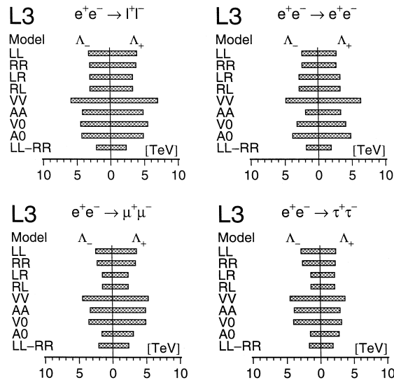
Fig. 3. One-sided 95% confidence level lower limits on the scale \Lambda_+ and \Lambda_- for contact interactions in leptonic channels. The limits correspond to the values given in Table 3.
