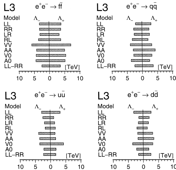
Fig. 2. One-sided 95% confidence level lower limits on the scales \Lambda_+ and \Lambda_- for contact interactions in hadronic channels and in all channels combined. The limits correspond to the values given in Table 2.
