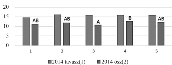
Figure 1: Effect of different fertilizer doses on soil carbon-dioxide emission ( \text{mg CO}_2 \times 100 \text{ g}^{-1} \times 10 \text{ day}^{-1} ) Spring(1), Autumn(2)
