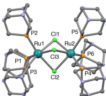
Figure 3. Ball and stick model of the [\{\text{Ru}(\text{PTA})_3\}_2(\mu\text{-Cl})_3]^+ cation in \mathbf{4}\cdot\mathbf{9H}_2\mathbf{O} with partial atom numbering scheme. Hydrogen atoms are omitted for clarity.
