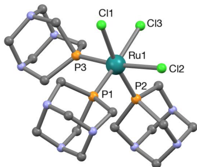
Figure 2. Ball and stick model of the fac -[RuCl 3 (HPTA) 3 ] 2+ cation in 3 ·HCl·2H 2 O with partial atom numbering scheme. Hydrogen atoms are omitted for clarity.
