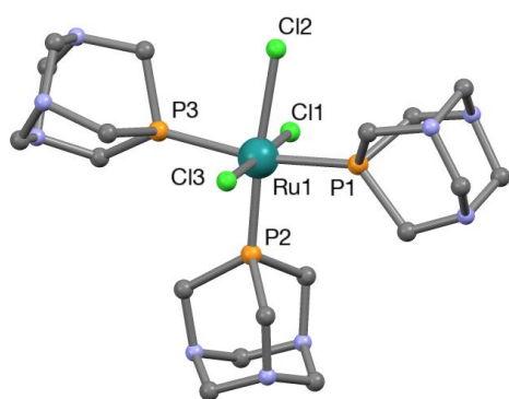
Figure 1. Ball and stick model of the mer -[RuCl 3 (HPTA) 3 ] 2+ cation in 2 ·1.25H 2 O with partial atom numbering scheme. Hydrogen atoms are omitted for clarity.
