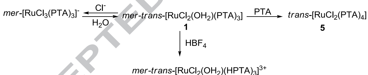
Scheme 3. Reactivity of mer-trans-[RuCl_2(OH_2)(PTA)_3] ( 1 ) in water towards PTA, HBF 4 and Cl - at room temperature
