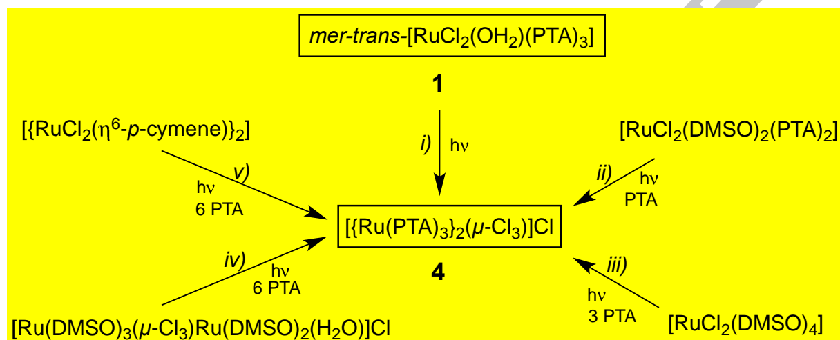
Scheme 6. Formation of [\{\text{Ru}(\text{PTA})_3\}_2(\mu\text{-Cl})_3]\text{Cl} ( 4 ) from various precursors at room temperature in water under illumination
