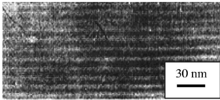
FIG. 1. Cross-sectional transmission electron micrograph (white and dark regions correspond to As_2S_3 and Se, respectively).
