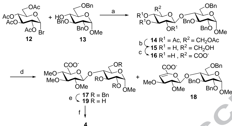
Scheme 1. Synthesis of the EF fragment of idraparinix by selective oxidation. Reagents and conditions: (a) CH_2Cl_2 -toluene, 4 Å Ms, AgOTf, -30^\circ C to rt, 24 h (94%); (b) MeOH, NaOMe, rt, 2 h (97%); (c) sat NaHCO_3 , KBr, NaOCl, TEMPO, 0^\circ C to rt, 2 h (78%); (d) DMF, NaH, MeI, 0^\circ C to rt, 2 h ( 17 : 42%, 18 : 40%); (e) ethanol, Pd(C), H_2 , 10 atm, rt, 12 h (94%); (f) DMF, SO_3 \cdot py , 0^\circ C to rt, 5 h (70%).
