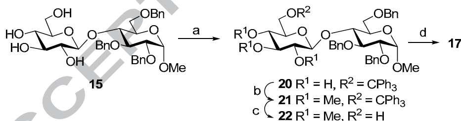
Scheme 2. Improved synthesis of the methylated uronate 17 . Reagents and conditions: (a) py, TrCl , 0^\circ C to rt, 24 h (83%); (b) DMF, NaH, MeI, 0^\circ C to rt, 2 h (86%); (c) 80% AcOH, 50^\circ C , 2 h (98%); (d) sat NaHCO_3 , KBr, NaOCl, TEMPO, 0^\circ C to rt, 2 h (64%).
