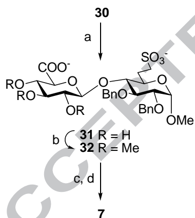
Scheme 5. Synthesis of the 6-deoxy-6-sulfonatomethyl analogue of the EF fragment of idraparinux by selective oxidation. Reagents and conditions: (a) sat \text{NaHCO}_3 , \text{KBr} , \text{NaOCl} , TEMPO, 0^\circ\text{C} to rt, 2 h (91%); (b) DMF, \text{NaH} , \text{MeI} , 0^\circ\text{C} to rt, 2 h (79%); (c) ethanol, \text{Pd(C)} , \text{H}_2 , 10 atm, rt, 12 h (96%); (d) DMF, \text{SO}_3\cdot\text{py} , 0^\circ\text{C} to rt, 5 h (65%).
