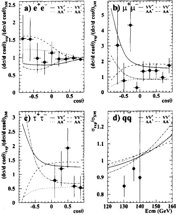
Fig. 2. Differential cross-sections normalised to the expectations of the Standard Model for the e^+e^- (a), \mu^+\mu^- (b), \tau^+\tau^- (c) and q\bar{q} (d) channels. The points with error bars are the present measurements and the curves indicate maximum deviations allowed at 95% confidence level for the W and AA models.
