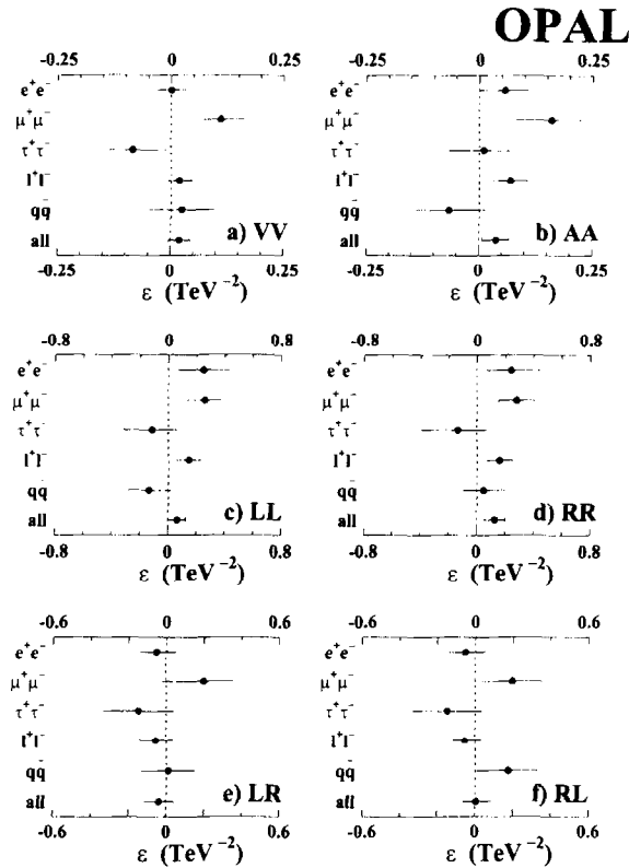
Fig. 1. Values of \varepsilon ( \text{TeV}^{-2} ) shown with one standard deviation errors for the six contact interaction models. The results for the leptonic channels are identical for the LR and RL .
