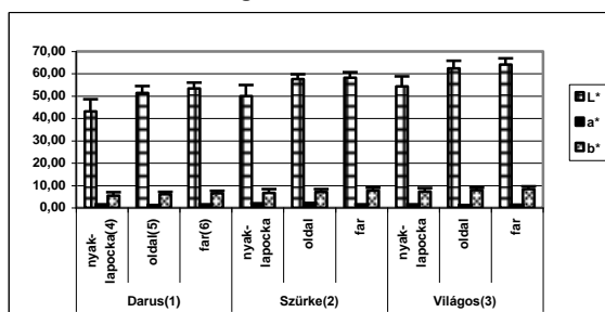
Figure 2: L^*a^*b^* values of crane, grey and light grey coat colour varieties in cows crane(1), grey(2), light grey(3), neck-shoulder(4), side(5), croup(6)
