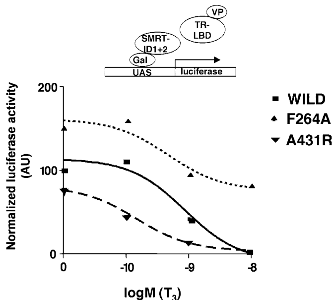
FIG. 7. Interaction of SMRT ID-1+2 with TR mutants containing mutations equivalent to RAR-LBD W225A and A392R. VP16 fusion proteins of hTRβ-LBD (wild type and F264A and A431R, equivalent to W225A and A392R in RARα) were tested for interaction with Gal-SMRT-ID-1+2 in mammalian two-hybrid analysis. Transient transfections of VP16 fusion hTRβ mutants were carried out in the presence of increasing amounts of triiodothyronine (T 3 ). The strength of interactions is expressed as normalized luciferase activity; representative experiments are shown. Curves were fitted by Prism (GraphPad Prism Software, Inc.). AU, arbitrary units.
