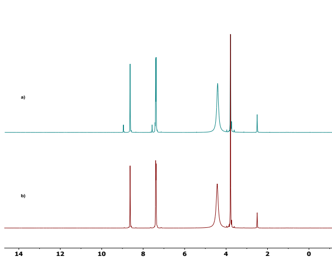
Fig. 12. 400 MHz ^1\text{H} NMR spectra of the material obtained by Method B in a mixture of \text{DMSO-}d_6 (0.3 ml) and \text{D}_2\text{O} (0.1 ml) a) 313 K; b) 323 K.
