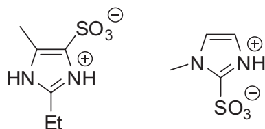
Fig. 2. Zwitterionic structures of sulfonated imidazoles [16,17].
