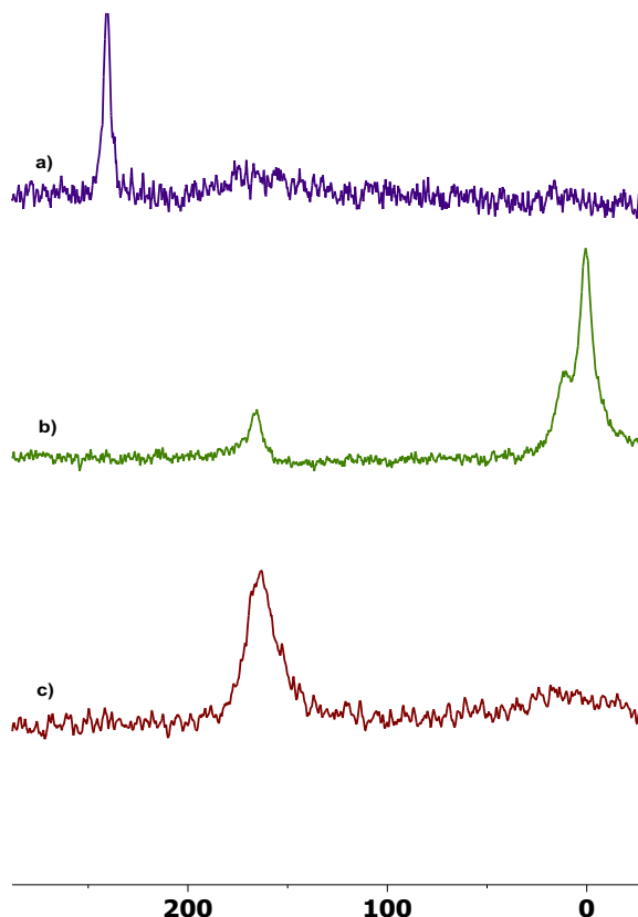
Fig. 13. 54.2 MHz 17 O NMR spectra without proton decoupling. a) neat [HMim][SO 3 Cl] ( 3 ) δ = 240.8 ppm, b) substance obtained by Method B in the presence of DMSO- d 6 and D 2 O (50 μL D 2 O, 298 K) δ = 165.5 ppm (HSO 4 − ), δ = 13.1 ppm (DMSO), and δ = 0.0 ppm (excess H 2 O was added as reference) and c) [HMim][HSO 4 ] ( 4 ) in the presence of DMSO- d 6 (50 μL) δ = 163.6 ppm.
