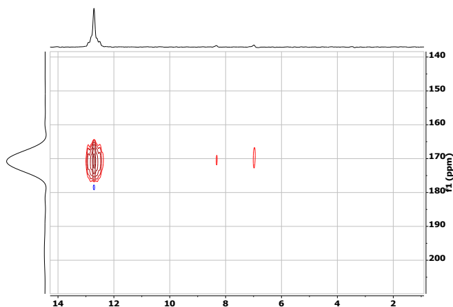
Fig. 7. Proton-detected ^{15}\text{N} - ^1\text{H} HSQC spectrum of a neat sample of compound 3 ( J = 110 \text{ Hz} ) (obtained by Method A).
