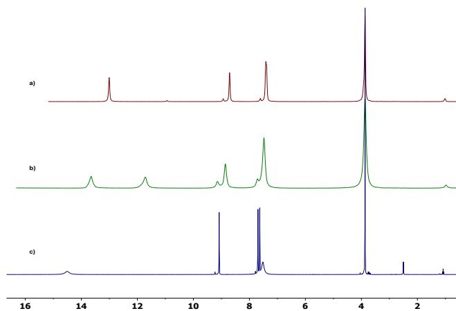
Fig. 11. a) 400 MHz ^1\text{H} NMR spectra of a neat sample prepared by Method A (300 K); b) ^1\text{H} NMR spectrum of the same sample after addition of 30% \text{DMSO-}d_6 (300 K); c) ^1\text{H} NMR spectrum of a diluted sample (70 mg / 0.4 ml \text{DMSO-}d_6 (300 K) (The shift of the methyl singlet in spectrum a) is adjusted to the same signals of the spectra obtained in \text{DMSO-}d_6 b).)
