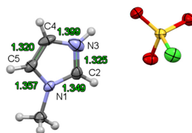
Fig. 3. X-ray structure of ionic liquid ([HMim][ \text{SO}_3\text{Cl} ]) (3) with partial numbering scheme and selected bond distances. S–O distances are in the range of 1.433–1.439 Å. Thermal ellipsoids drawn at 50% probability.
