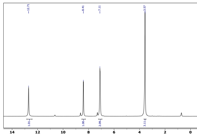
Fig. 4. ^1\text{H} -400 MHz NMR spectrum of a neat sample of compound 3 (obtained by Method A).
