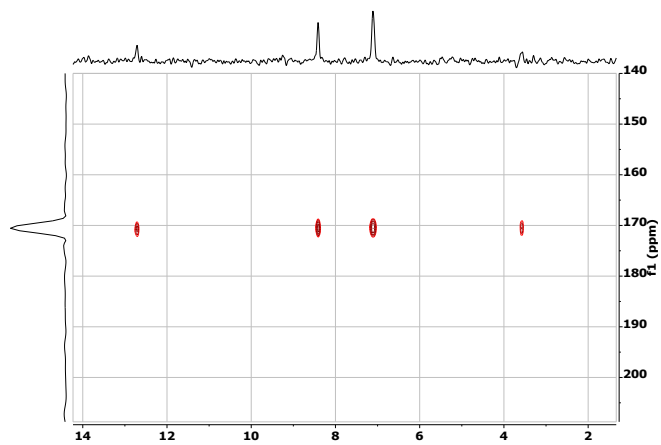
Fig. 8. Proton-detected ^{15}\text{N} - ^1\text{H} HSQC spectrum of a neat sample of compound 3 ( J = 11 \text{ Hz} ) (obtained by Method A).
