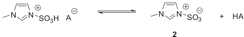
Scheme 1. Possible deprotonation the N -sulfonated cation ([MSim] + ) in the presence of anions
