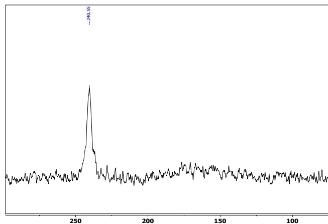
Fig. 9. ^{17}\text{O} -direct detection (zg) not-proton decoupled (linewidth \sim 300 \text{ Hz} ) NMR spectrum of a neat sample of compound 3 (obtained by Method A).
