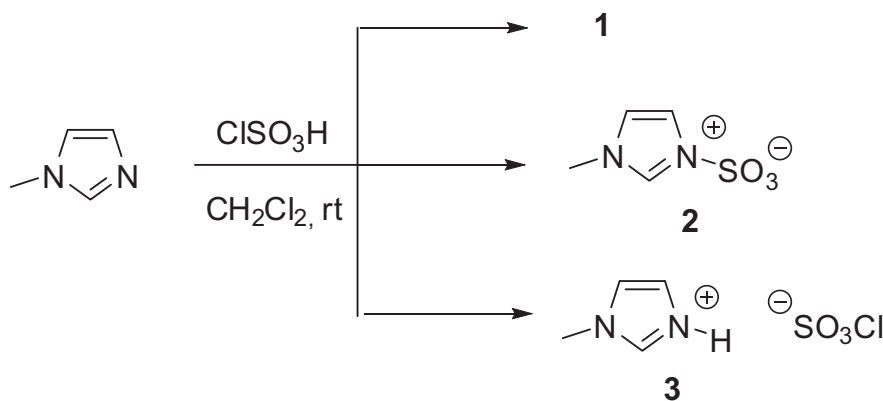
Scheme 2. Possible products of the reaction of 1-methylimidazole with chlorosulfonic acid
