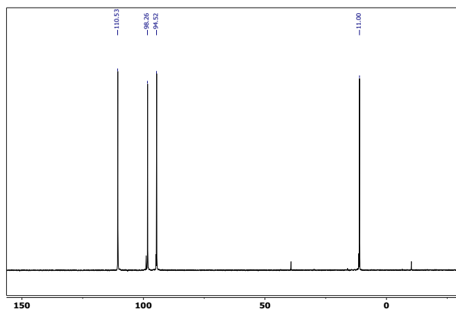
Fig. 5. ^{13}\text{C}\{^1\text{H}\} - 100.3 MHz NMR spectrum of a neat sample of compound 3 (obtained by Method A).
