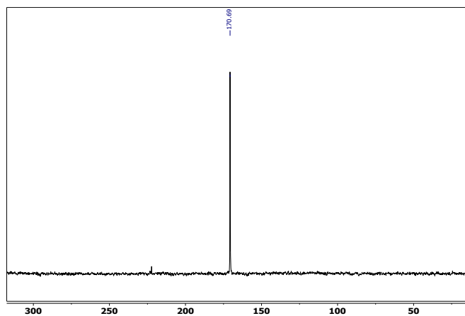
Fig. 6. ^{15}\text{N}\{^1\text{H}\} inverse-gated- spectrum of a neat sample of compound 3 (obtained by Method A).
