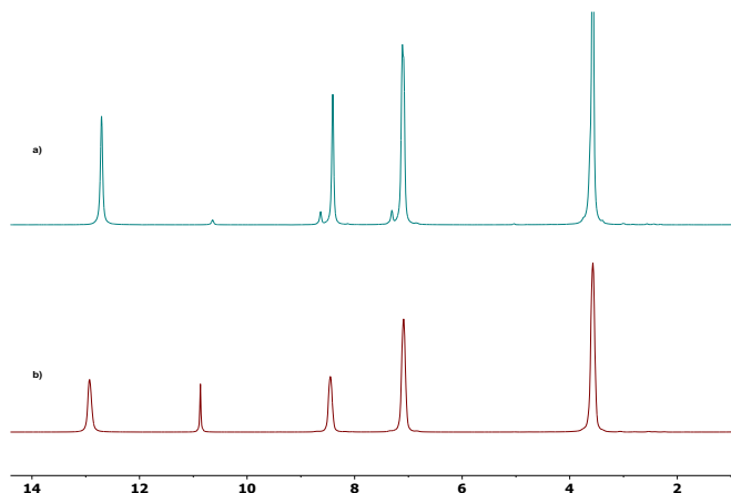
Fig. 10. a) 400 MHz ^1\text{H} NMR spectra of a freshly made neat sample prepared by Method B (300 K); b) ^1\text{H} NMR spectrum of the same sample after a two-month storage (304 K).
