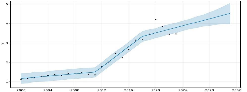
Figure 5: Original data, prediction domain, and predicted values using Prophet
