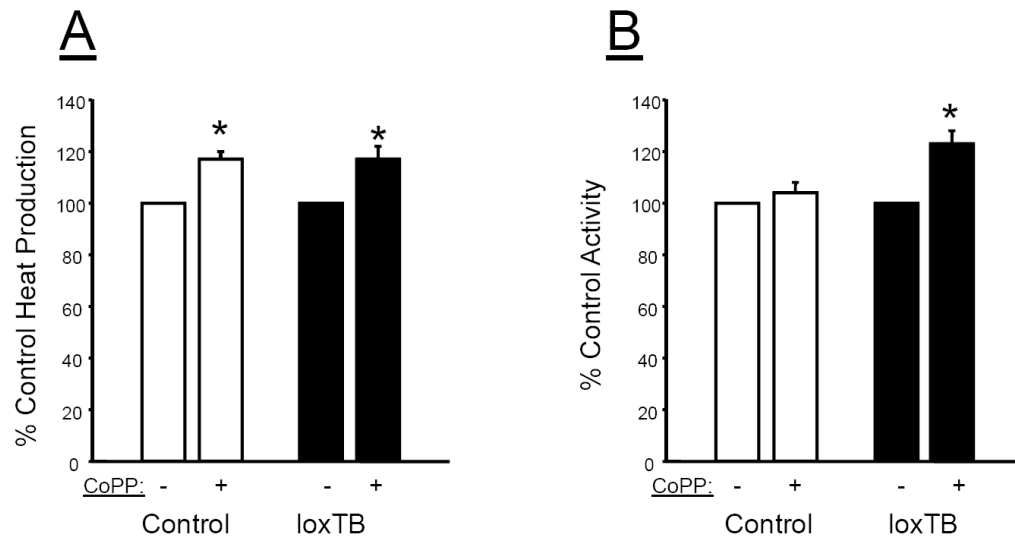
Figure 5. Effect of chronic CoPP treatment on A) 24 hour heat production and B) 24 hour locomotor activity in control C57 and loxTB mice. * = P < 0.05 as compared to corresponding value in non-CoPP treated mice, n=4 /group.
