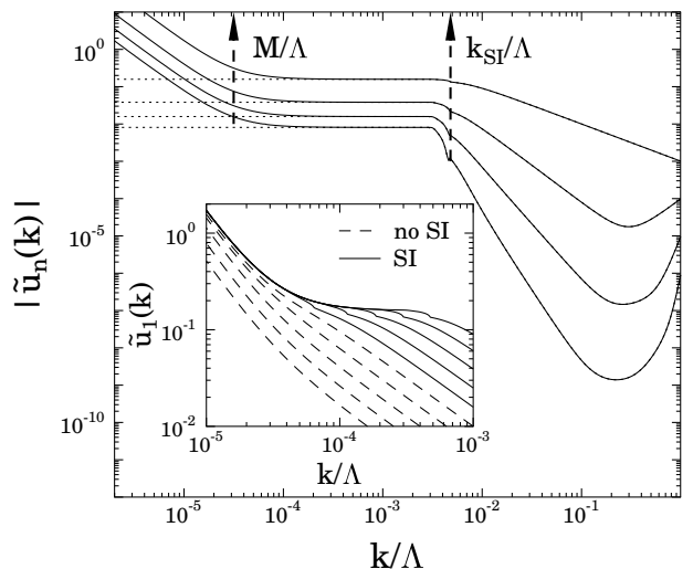
FIG. 2: RG flow of \tilde{u}_1, \dots, \tilde{u}_4 for \beta^2 = 4\pi and M^2 = 10^{-9}\Lambda^2 (solid line) or M^2 = 0 (dotted line). The scales of the spinodal instability k_{\text{SI}}/\Lambda and the mass M/\Lambda are indicated. The inset shows RG flows of \tilde{u}_1 for several different initial values at M^2 = 10^{-9}\Lambda^2 .
