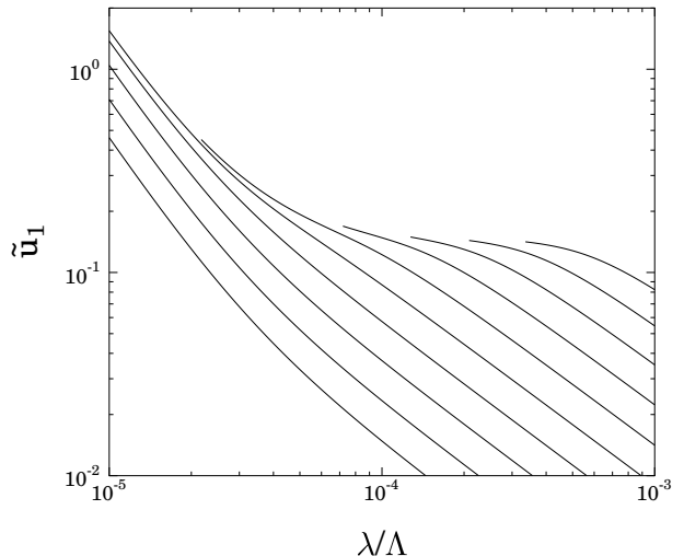
FIG. 6: Internal-space RG evolution of the coupling \tilde{u}_1 for several different initial values at M^2 = 10^{-9}\Lambda^2 .
