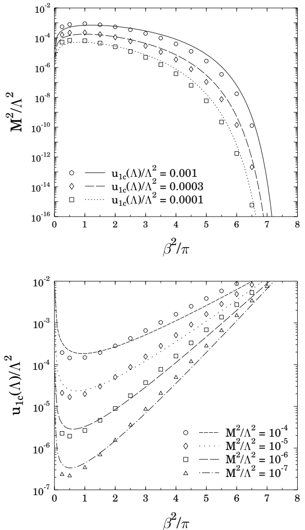
FIG. 3: The region with spinodal instability. Different symbols show the boundary obtained by the numerical computation with 10 coupling constants and the lines show the results obtained by taking into account a single Fourier mode only.
