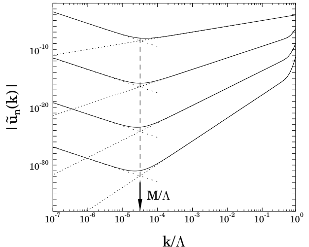
FIG. 1: RG flow of \tilde{u}_1, \dots, \tilde{u}_4 for \beta^2 = 12\pi and M^2 = 10^{-9}\Lambda^2 (solid line) or M^2 = 0 (dense dotted line). The plot also shows the asymptotic IR scaling \sim k^{-2} (rare dotted line). The massive and the massless flows depart at the scale M , indicated by a dashed vertical line, placed at the intersection of the dotted lines.
