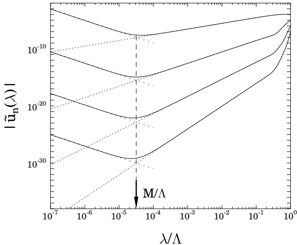
FIG. 5: RG flow of \tilde{u}_1, \dots, \tilde{u}_4 for \beta^2 = 12\pi and M^2 = 10^{-9}\Lambda^2 (solid line) or M^2 = 0 (dense dotted line). The plot also shows the asymptotic IR scaling \sim \lambda^{-2} (rare dotted line). The massive and the massless flows depart at the scale M , indicated by a dashed vertical line, placed at the intersection of the dotted lines.
