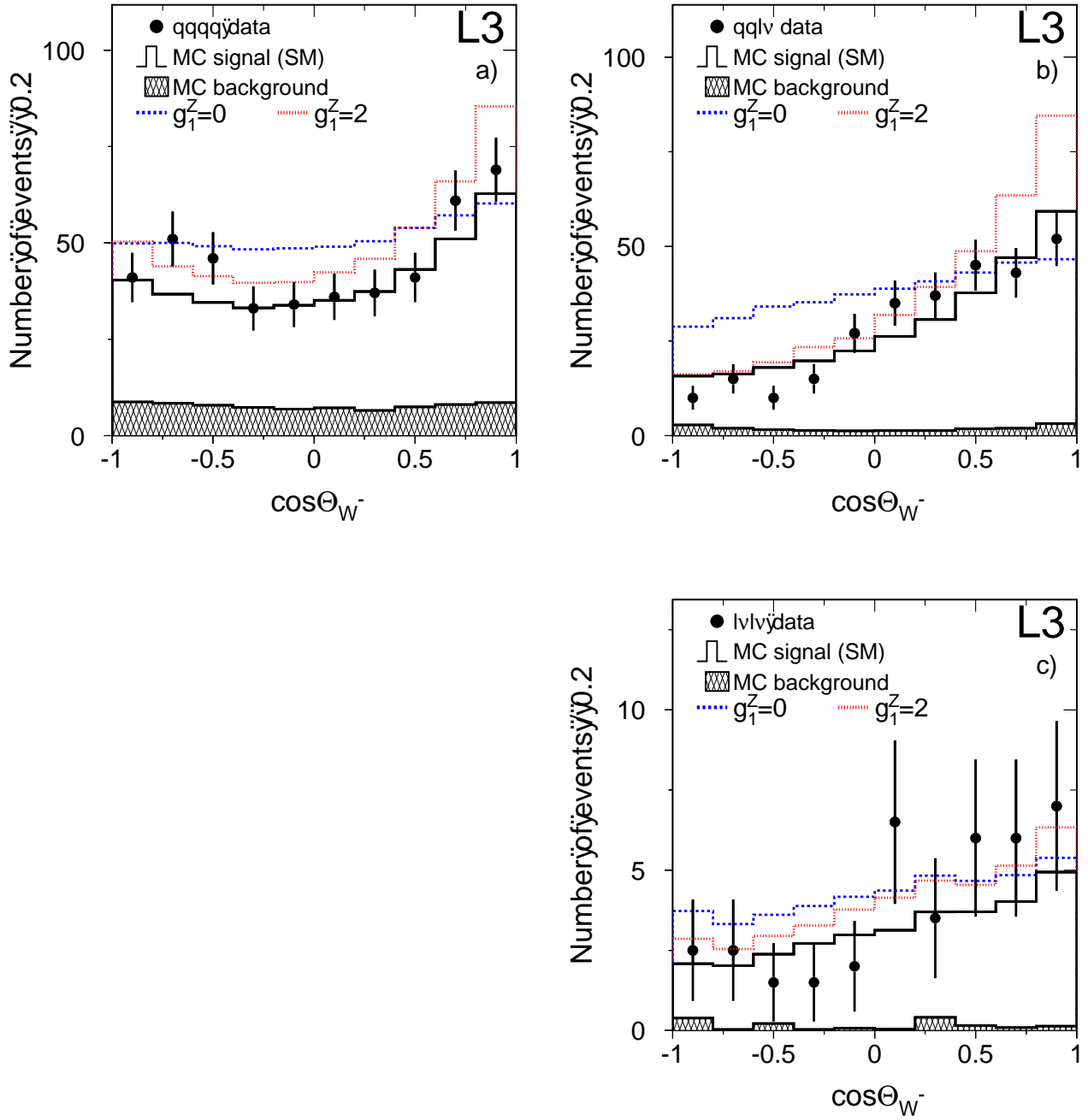
Figure 1: Distributions of the reconstructed polar scattering angle, \cos\Theta_{W^-} , of the W^- boson in W -pair events for a) qq\bar{q}\bar{q} , b) qql\nu , c) l\nu l\nu events. The data collected at \sqrt{s} = 183 GeV are shown, together with the expectations for the SM ( g_1^Z = 1 ), and for anomalous TGCs ( g_1^Z = 0 or 2). For l\nu l\nu events, both solutions enter with a weight of 0.5.
