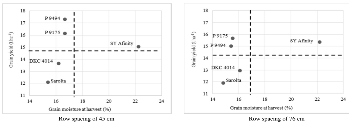
Figure 2: Relationship between yield amount ( t\ ha^{-1} ) and its moisture content (%) by row spacings of 45 and 76 cm in the crop year of 2014 (Debrecen – Látókép 2014)
