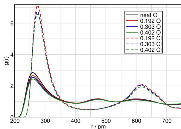
Fig. 5 Chloride mole fraction dependent H2-O/Cl RDFs of [C 4 C 1 Im][OTf]/[Cl]. Please note, for clarity we show only a range, the full functions can be found in the SI. These decay properly to 1.
