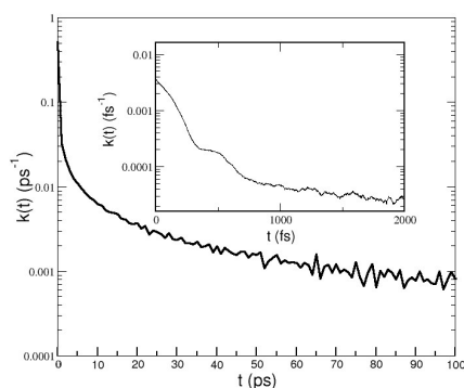
Fig. 6 Semi-log plot of the rate function k(t) for the ion pair process in [C_4C_1Im][Br] . In the analysis the long trajectory was selected. The inset shows the analysis of the 200 ps trajectory, obviously at 0.35 - 0.5 ps a transient period is visible.
