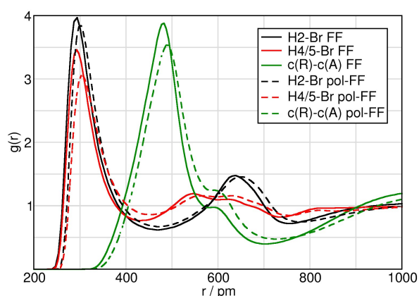
Fig. 2 Cation-anion radial distribution functions (RDFs). Black: H2; red: H4/5; dark green: RDFs between centre of ring c(R) and centre of mass anion c(A). Solid line: standard force field; dashed line: polarizable force field. Please note, for clarity we show only a range of the RDF, the full functions can be found in the SI, these decay properly to 1.
