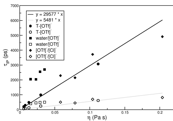
Fig. 9 Correlating calculated \tau^{\text{IP}} (ps) with experimental viscosities (Pa s). Zero intercept is enforced in this fit. Correlation coefficients are 0.859 and 0.821 for the intermittent and the reactive flux lifetimes, respectively.
