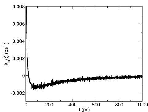
Fig. 7 The restricted rate function k_{in}(t) for the ion pair process in [C_4C_1Im][Br] . In the analysis the long trajectory was selected.
