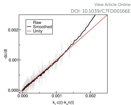
Fig. 8 Correlation plot for the ion pair process in [C_4C_1Im][Br] . Both axes are in ps^{-1} . In the analysis the long trajectory was selected. The fit to the line with unity slope was carried out from 160 to 8000 ps the values obtained for k_f and k_b are 0.019 ps^{-1} and 0.005 ps^{-1} , see also table 5.
