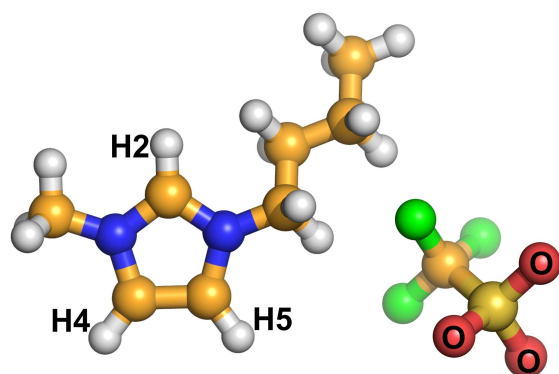
Fig. 1 Labelling as used in the article. Left: 1-butyl-3-methylimidazolium cation and right: trifluoromethanesulfonate (triflate, [OTf] - ) anion. (Brown: carbon; blue: nitrogen; white: hydrogen; red: oxygen; yellow: sulphur; green: fluorine)
